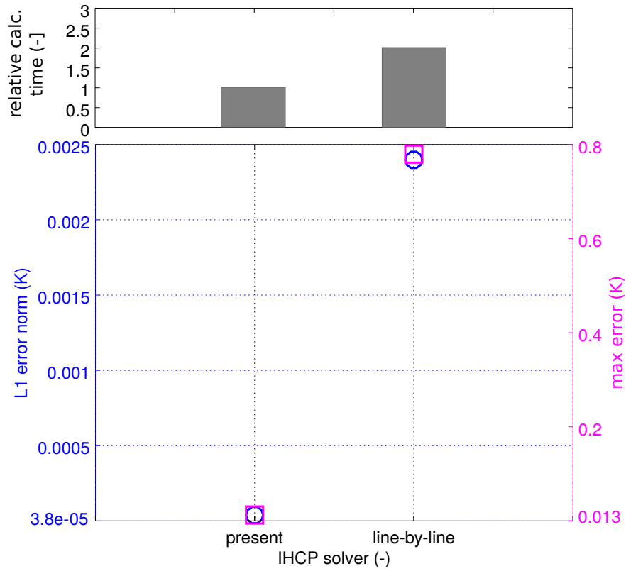
FIGURE 16. Results ( HTC_t ) of the proposed (OpenFOAM ® ) and the line-by-line IHCP solver.
