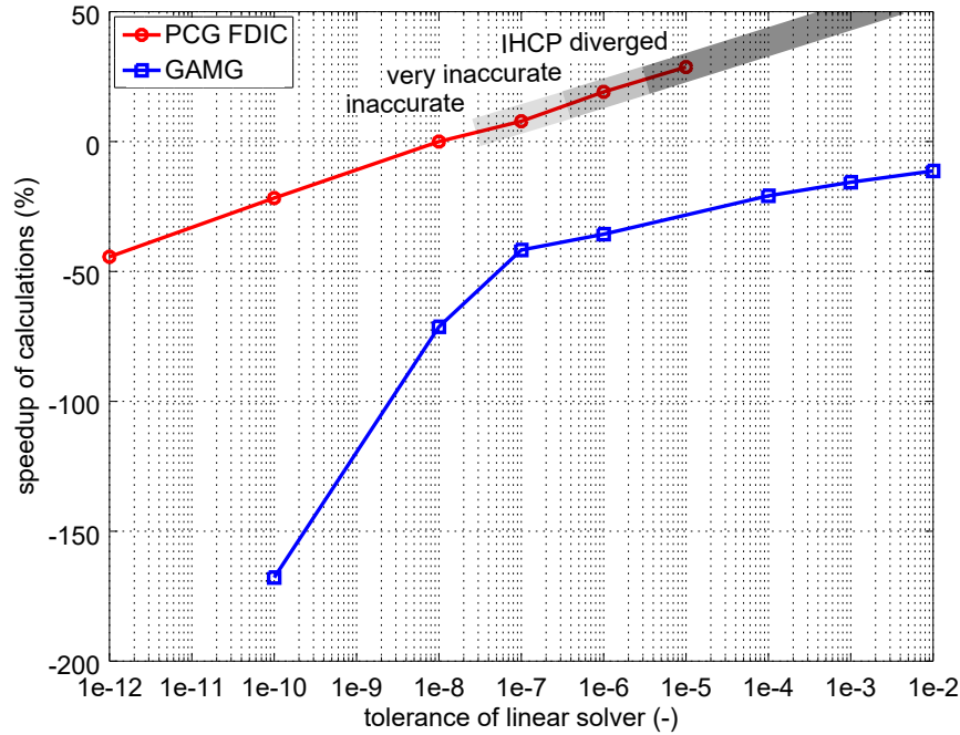
FIGURE 14. Performance comparison of the preconditioned (FDIC) conjugate gradient (PCG) method and the multigrid (GAMG) solver from the OpenFOAM® CFD package for the IHCP with 4k finite volume elements.
