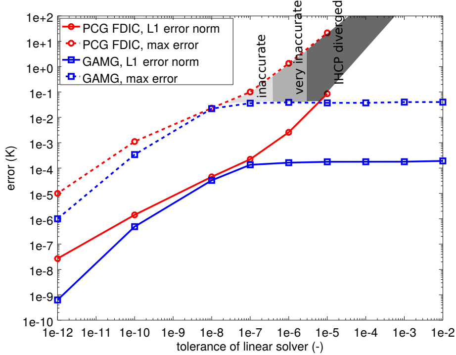
FIGURE 15. Convergence of the preconditioned (FDIC) conjugate gradient (PCG) method and the multigrid (GAMG) from the OpenFOAM® CFD package from the perspective of L^1 (solid curves) and max errors (dashed curves) for the IHCP with 4k finite volume elements.
