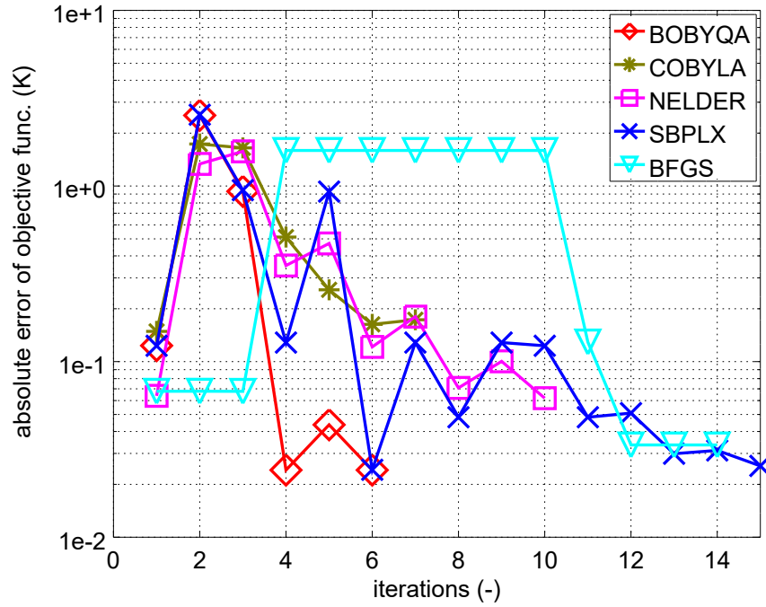
FIGURE 13. An example of the iteration process of the minimizers considered in the present study.
